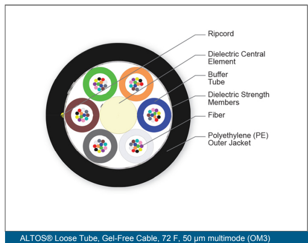
ALTOS® Loose Tube, Gel-Free Cable, 72 F, 50 µm multimode (OM3)
