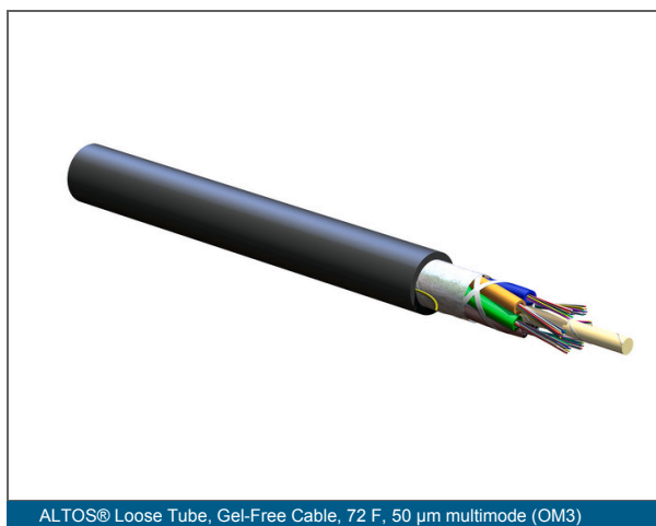
ALTOS® Loose Tube, Gel-Free Cable, 72 F, 50 µm multimode (OM3)
